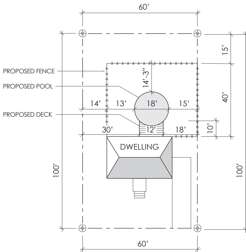
SITE PLAN EXAMPLE - PROPOSED POOL, DECK & FENCE
