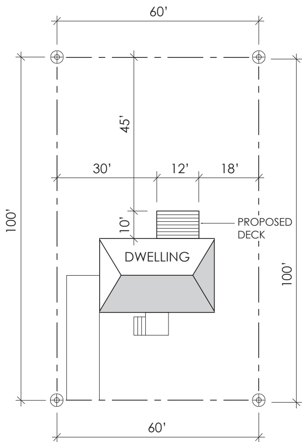
SITE PLAN EXAMPLE - PROPOSED DECK
