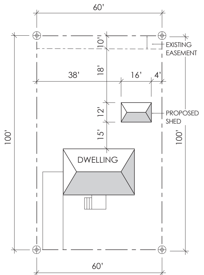
SITE PLAN EXAMPLE - PROPOSED SHED
