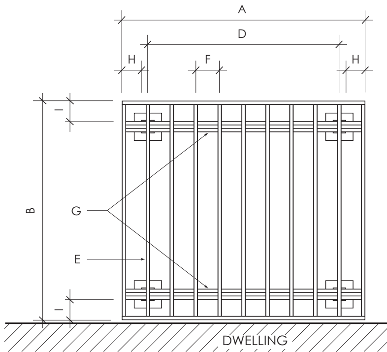
TYPICAL DETACHED DECK PLAN
