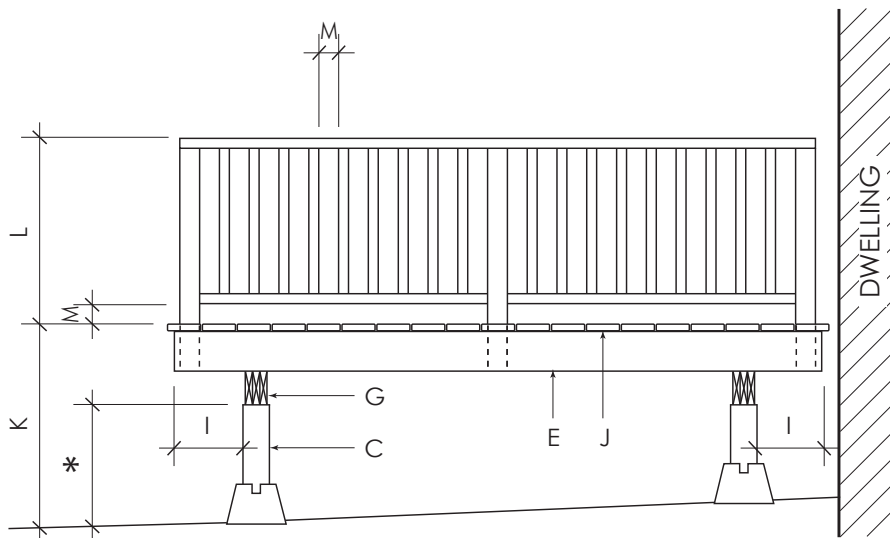
TYPICAL DETACHED DECK SECTION
